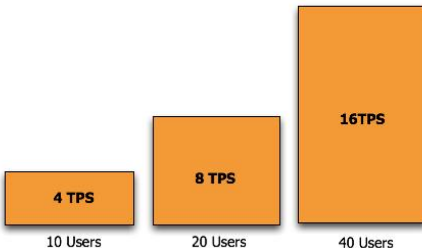
Throughput Increases Proportionately To The Number of Concurrent Users In Linear Scalability
